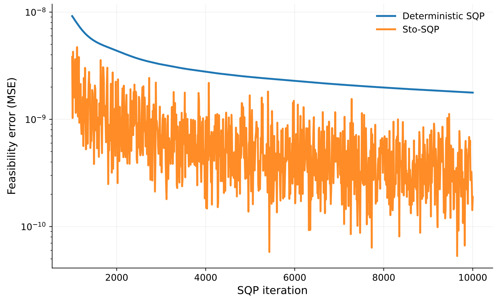
Burgers equation: feasibility error — zoom: iter \geq 1000
